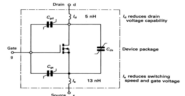
Figure 4.11. MOSFET equivalent circuit including terminal voltage dependent capacitance and inductance for the TO247 package.
