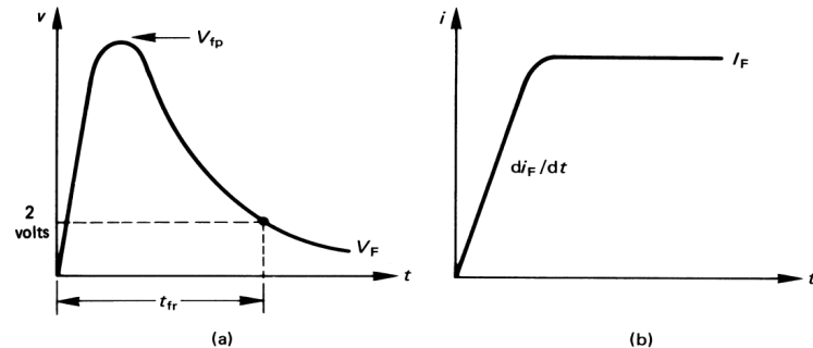
Figure 4.2. Diode forward recovery measurement:
