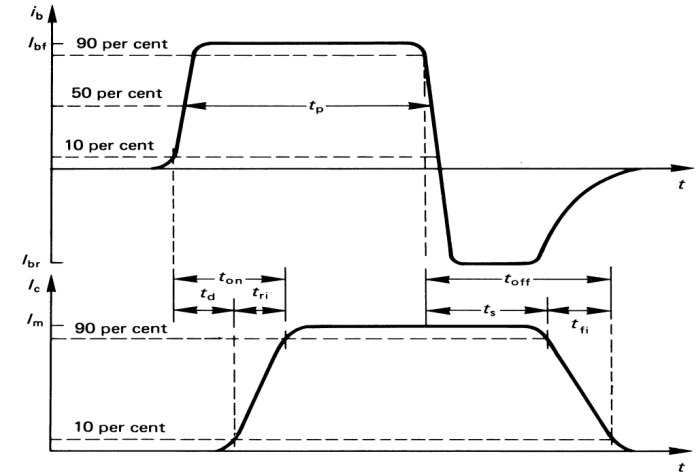
Figure 4.9. Defining transistor base and collector current switching times for turn-on and turn-off.
