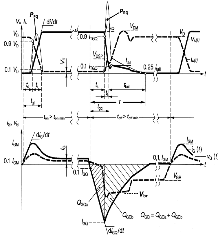
Figure 4.18. Schematic representation of GTO thyristor turn-off waveforms.
