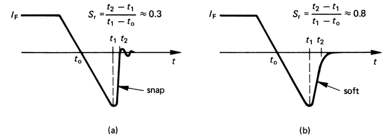
Figure 4.5. Comparison of fast recovery diode di_r/dt characteristics of: (a) short current tail, producing snap-off (low S_r ) and (b) gradual current tail, producing soft recovery (high S_r ).
