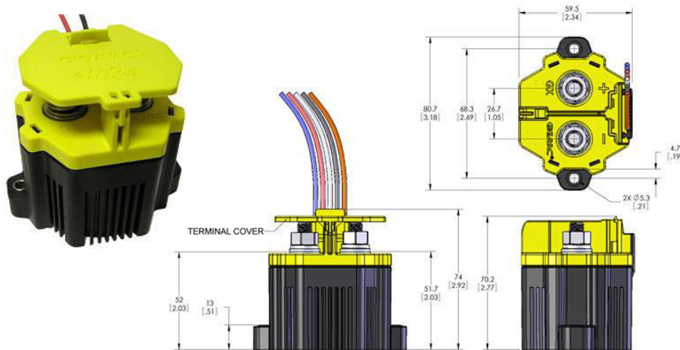
Figure 33.32. Typical 750V dc 350A dc relay.
