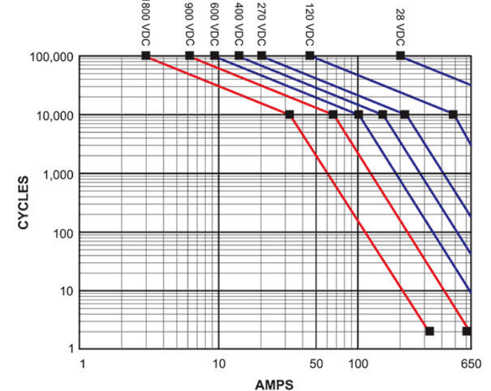
Figure 33.33. HV dc relay; upper V-I resistive load make and break limits and life cycling ratings.
