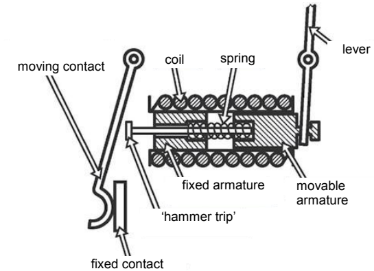
Figure 33.13. Magnetic trip unit of an MCB.
