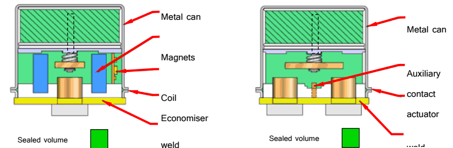
Figure 33.26. Sealed ceramic encapsulated dc relay.
