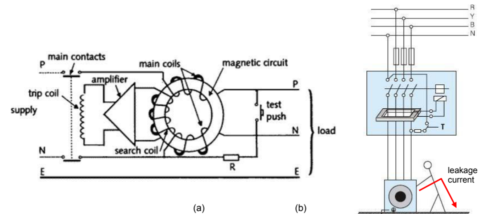
Figure 33.19. RCCB detection types: (a) single phase and (b) three phase.
