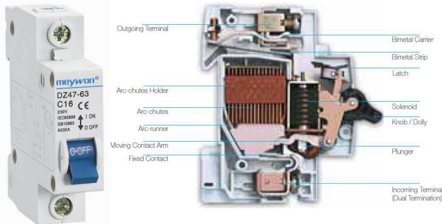
Figure 33.12. Miniature circuit breaker.
