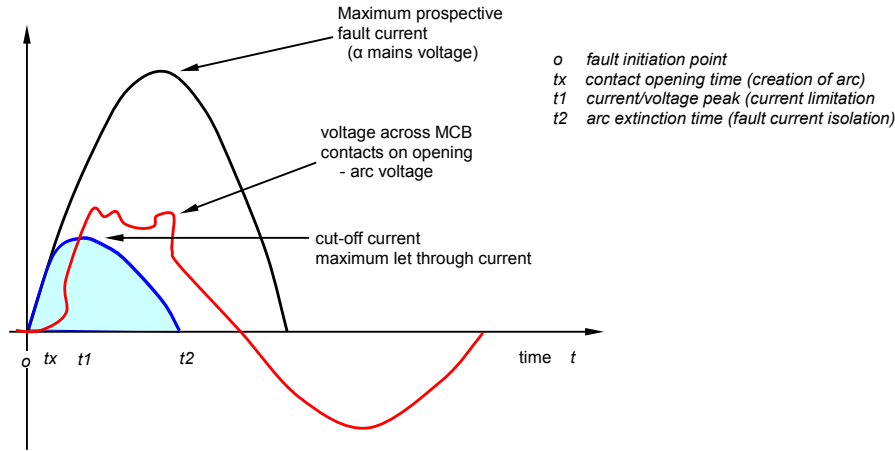
Figure 33.15. Current limiting effect of an MCB.
