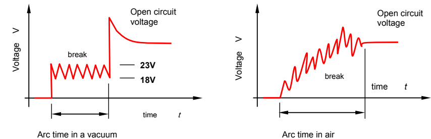
Figure 33.22. Comparison of arcs in air and a vacuum.
