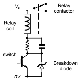
Figure 33.8. Reduction of relay activation time.
