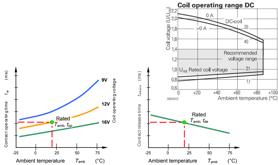
Figure 33.4. Contact operate and release time dependence on coil temperature.
