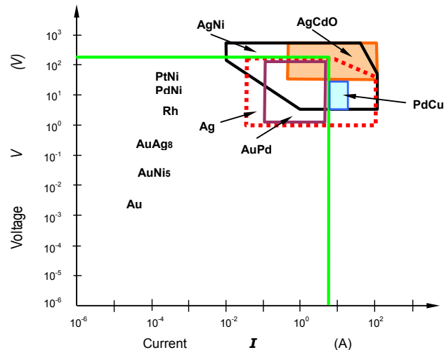
Figure 33.1. Low voltage and current contact materials.
