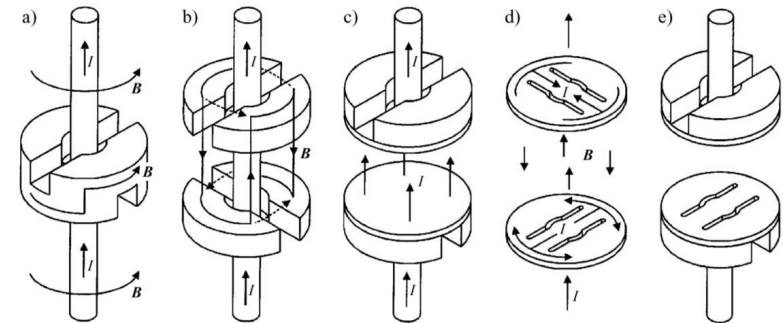
Figure 33.37. Basic principle of a quadruple axial magnetic field contact: (a) ferromagnetic circuit arrangement; (b) magnetic circuit in an open position; (c) contact system, without electrical pole face slots; (d) electrical pole face electrode slots; and (e) electrical plus magnetic combined quadrupolar contact systems.
