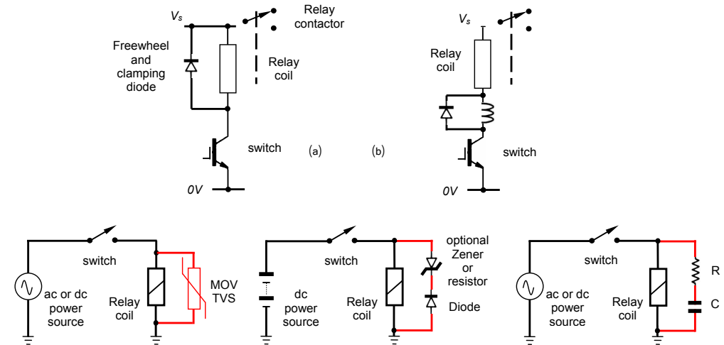
Figure 33.6. Various relay coil voltage suppression techniques.
