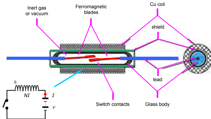
Figure 33.27. A reed relay consisting of a wound coil with a reed switch.
