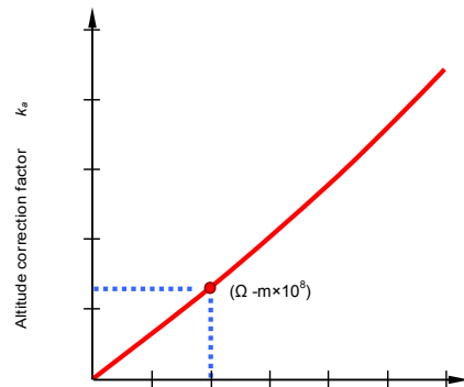
Figure 33.41. Graph for determining the voltage correction factor k_a according to the altitude.
