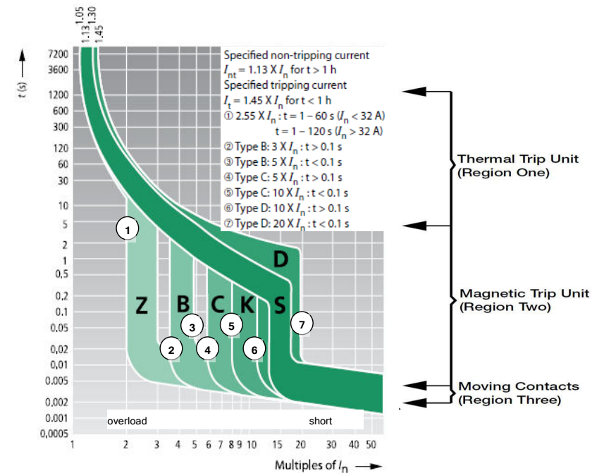
Figure 33.14. MCB characteristic curves.
