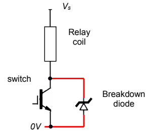
Figure 33.5. Indirect coil voltage suppression.
