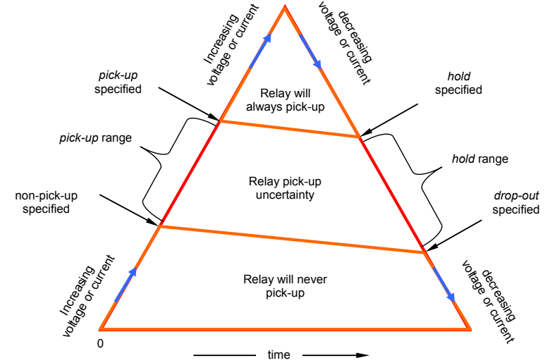
Figure 33.3. Graphical presentation of relay performance related definitions.
