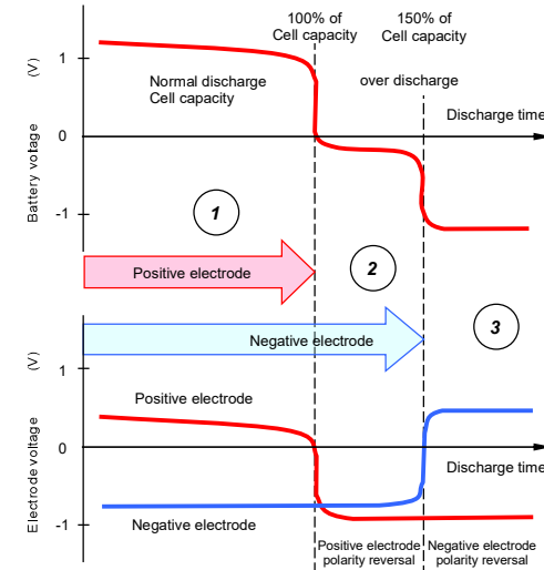
Figure 28.32. NiCd discharge polarity reversal characteristics.
