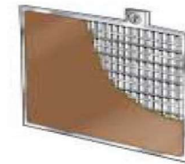
Figure 28.8. Rod plate structure with paste filling.
