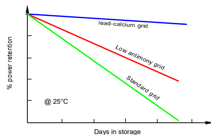
Figure 28.4. Self-discharge rates of different plate materials.
