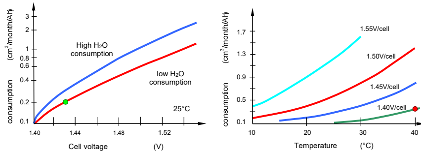
Figure 28.30. NiCd discharge water consumption for different voltages and different (a) plate types and (b) temperatures.
