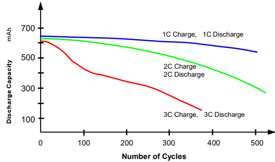
Figure 28.42. Cycle/Lifetime of a lithium-ion cell as a function of charge and discharge rates.
