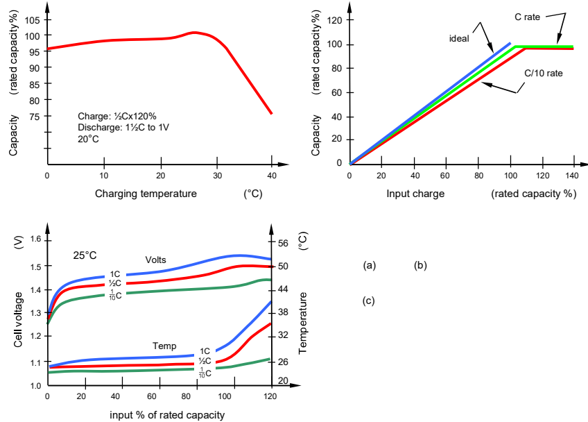
Figure 28.35. Effect of charge temperature and charge rate on charge capacity.
