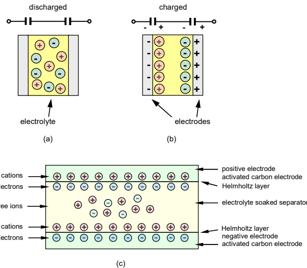
Figure 28.47. Supercapacitor (EDLC) showing formation of the double charge boundary layers: (a) discharged state; (b) fully charged state; and (c) partially discharged.
