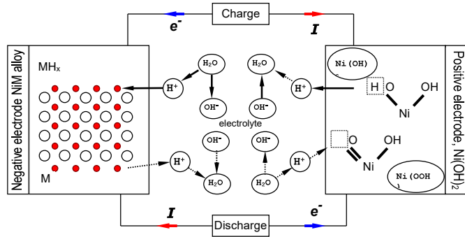
Figure 28.34. NiMH cell transport diagram for NiMH charging and discharging.
