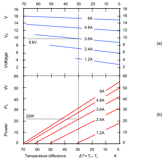
Figure 28.66. TEC performance curves: (a) upper plot \Delta T versus Voltage and (b) lower plot, \Delta T versus P_c .
