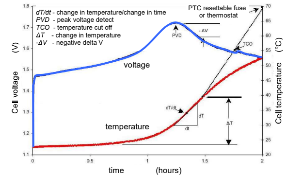
Figure 28.28. NiCd charge termination terminology.
