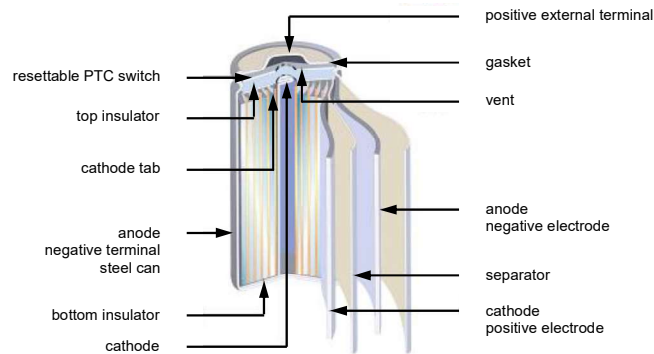
Figure 28.39. Spiral Cylindrically Wound Electrodes.
