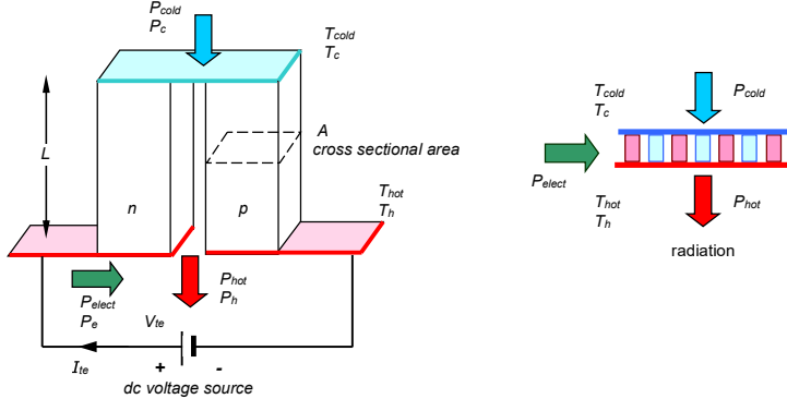
Figure 28.63. The thermoelectric couple based on the Peltier effect.
