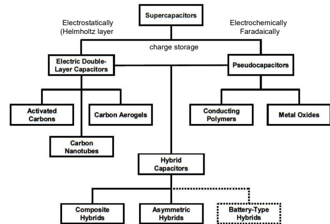
Figure 28.57. Supercapacitor family tree.
