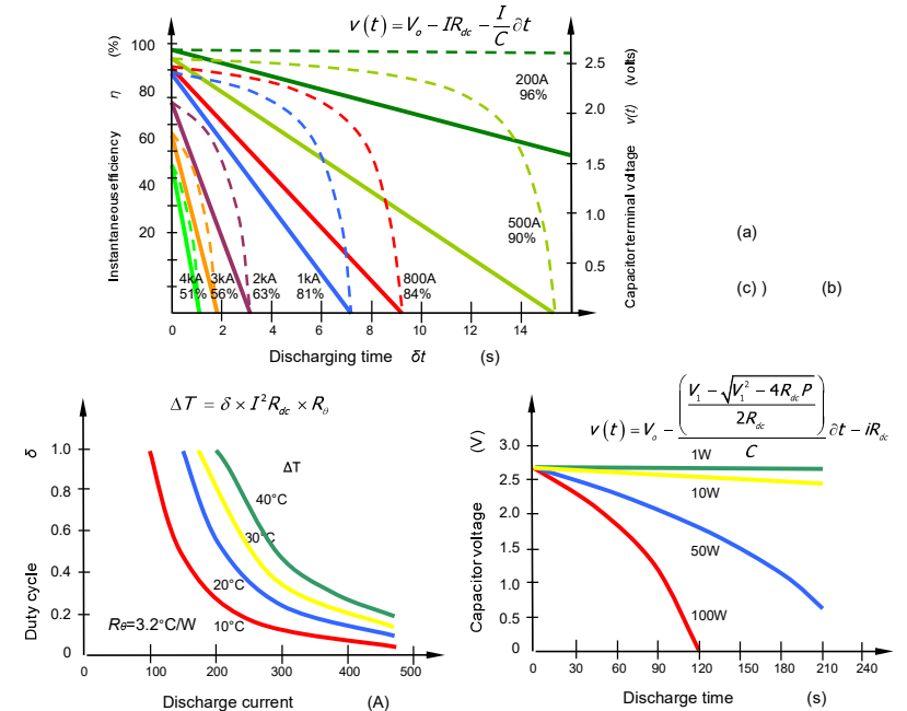
Figure 28.53. Supercapacitor 3000F, 2.7V, 0.29mΩ cell performance characteristic profiles: (a) constant current discharge, (b) constant power discharge, and (c) thermal dissipation with free convection in a 25°C ambient.
