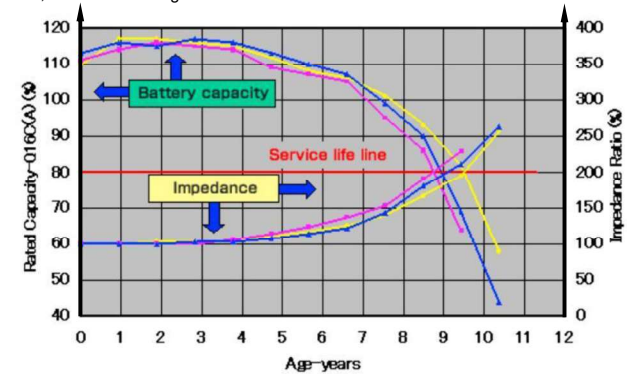
Figure 28.21. Battery impedance increase over battery lifetime.
