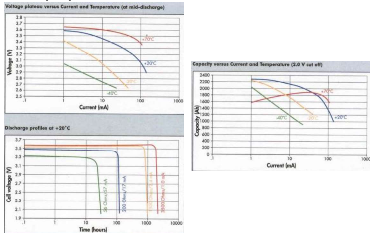
Figure 28.43. Li-ion cell capacity factors.
