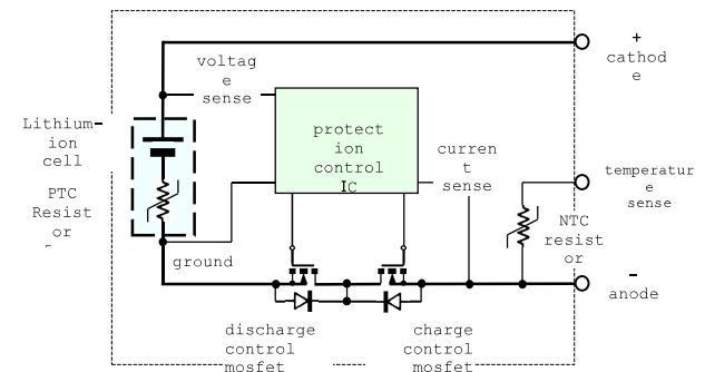
Figure 28.46. Protection circuitry for series connected double layer cells and Li-ion cells.
