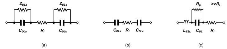
Figure 28.49, Derivation of the electrical equivalent circuit of the double-layer super-capacitor: (a) electrode-solution interface capacitance and impedances; (b) double-layer capacitances and electrolyte resistance; and (c) R-C series equivalent circuit model, with equivalent series inductance.
