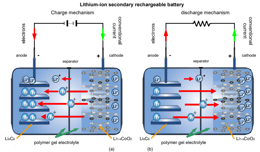
Figure 28.1. Cells charge mechanism and discharge mechanism.
