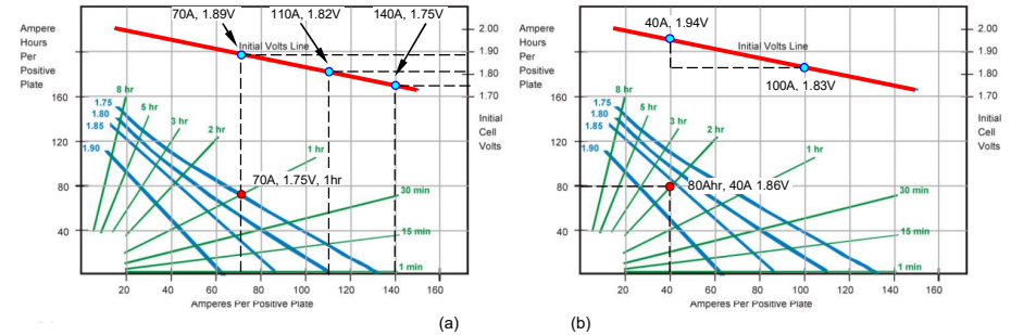
Figure 28.18. Typical battery discharge characteristics, for Example 28.1.
