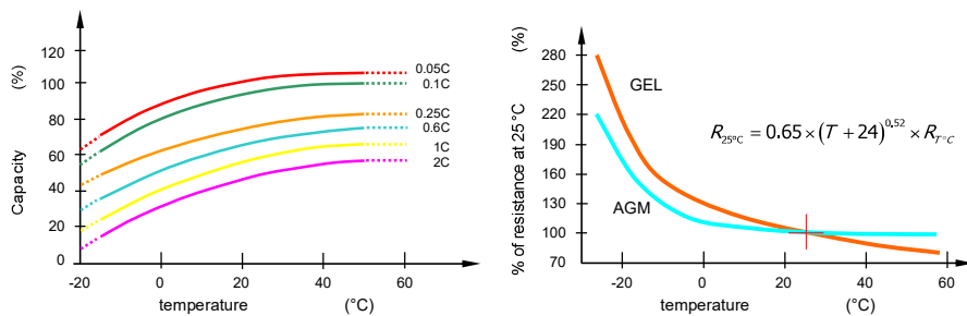
Figure 28.23. Effect of temperature on capacity and internal resistance.
