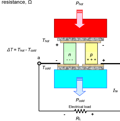
Figure 28.67. Single thermoelectric couple where T_{hot} > T_{cold} .
