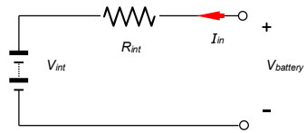
Figure 28.73. Battery model.
