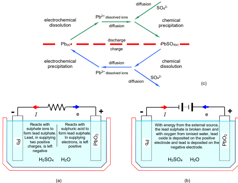
Figure 28.11. Lead acid battery plate reaction when being: (a) discharged, (b) charged, and (c) charge/discharge processes in the lead negative anode.
