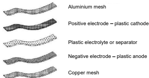
Figure 28.41. Lithium polymer cell construction layers.
