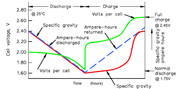
Figure 28.12. Electrolyte specific gravity of a lead acid cell during discharge, then charging.
