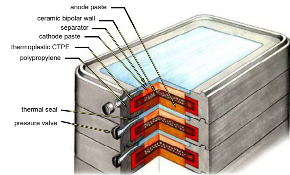
Figure 28.14. Construction of the bipolar lead-acid battery.
