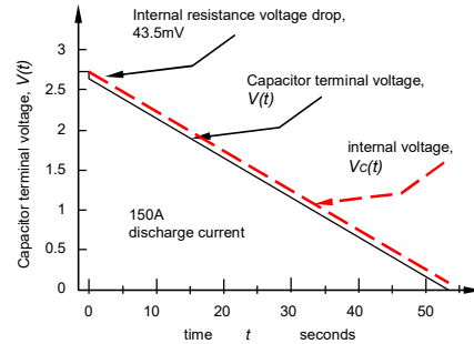
Figure 28.58. Solution to Example 28.7.
