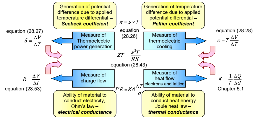
Figure 28.70. Thermoelectric characteristics summary.
