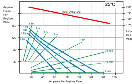
Figure 28.17. Typical battery discharge characteristics.
