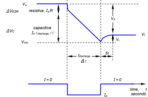
Figure 28.50. Voltage-time discharge profile of a supercapacitor.
