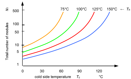
Figure 28.69. The total number of 127-couple, 6A Modules required for a 12V, 1A thermoelectric power generator.
