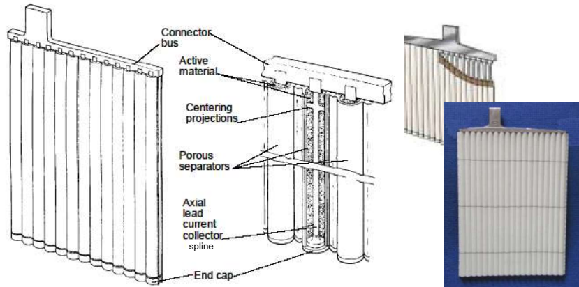
Figure 28.6. Tubular plate structure and paste filling.
