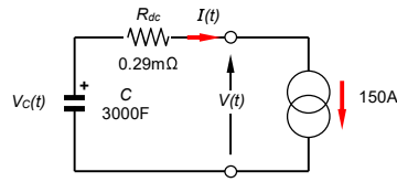
Figure 28.58. Solution to Example 28.7.
