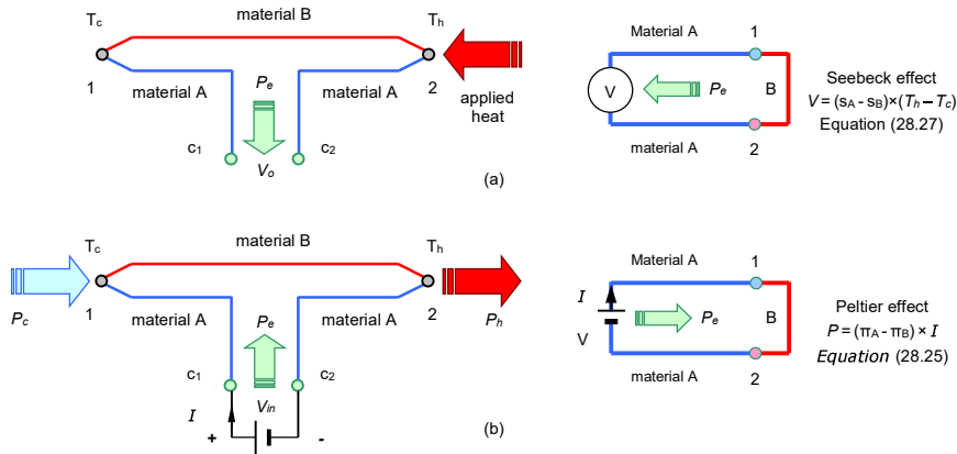
Figure 28.59. The (a) Seebeck and (b) Peltier effects.
