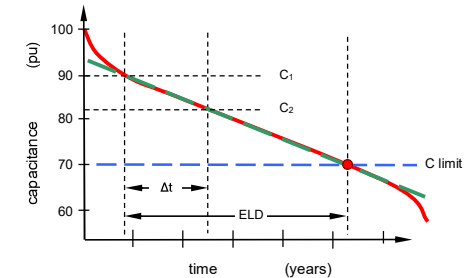
Figure 28.55. Supercapacitor lifetime determination.
