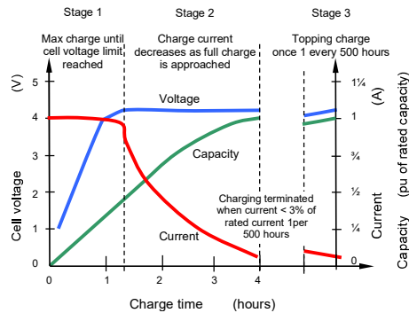
Figure 28.44. Charge stages of a Li-ion battery.
