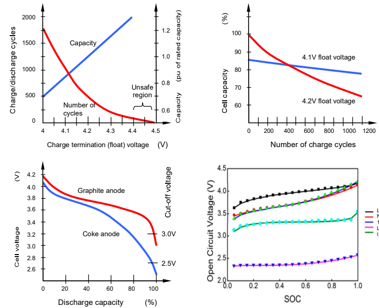
Figure 28.45. Li-ion charge float voltage and SOC characteristics.
