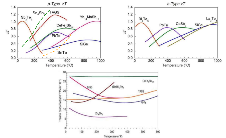
Figure 28.62. Performance of thermoelectric materials at various temperatures. TAGS (Te-Ag-Ge-Sb)
