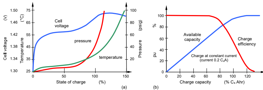
Figure 28.29. Charge characteristics of a NiCd cell: (a) the cell voltage, pressure and temperature characteristics are similar to a NiMH cell and (b) charge efficiency as a function of state of charge.
