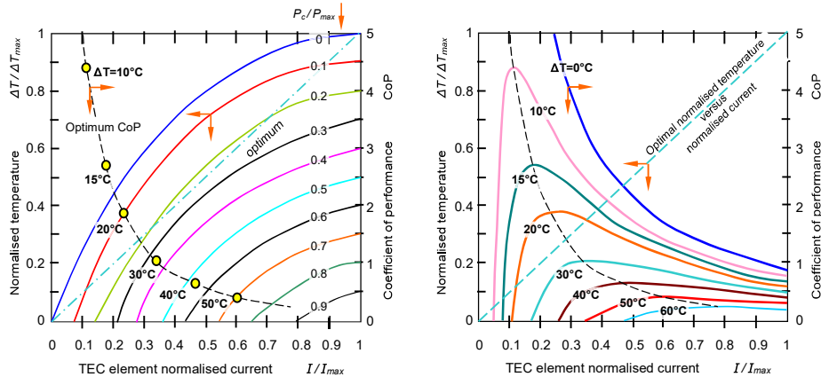
Figure 28.64. TEC:
