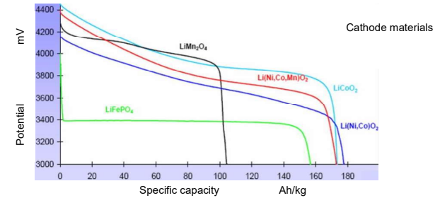
Figure 28.38. Comparison of cathode materials.
