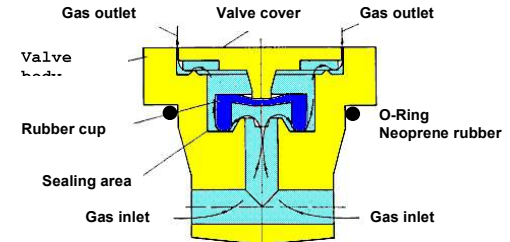
Figure 28.9. Valve system for sealed batteries.
