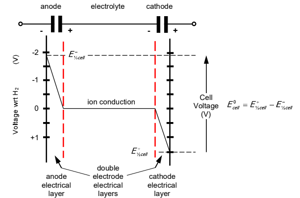
Figure 28.48. Voltage potential profile across the battery cell, fuel cell or electrochemical capacitor, where the structure and composition of the electrical double layers differ at the anode and cathode.
