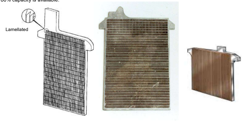
Figure 28.5. Planté grid structure and active paste filling.
