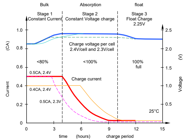
Figure 28.15. Charge stages of a lead acid battery; constant-current charge, topping charge, and float charge.
