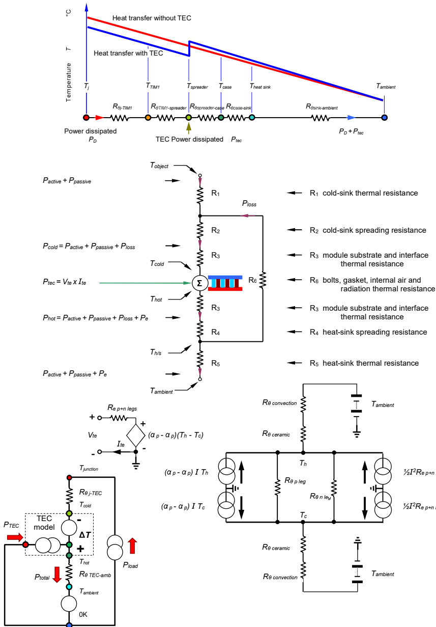
Figure 28.65. TEC cooling models: (a) thermal resistance model; (b) equivalent electrical circuit models; & (c) PSpice electrical model.
