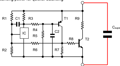
Figure 28.56. Supercapacitor voltage balancing circuit.
