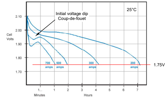
Figure 28.16. Cell voltage during discharge with a 1.75V/cell end voltage.
