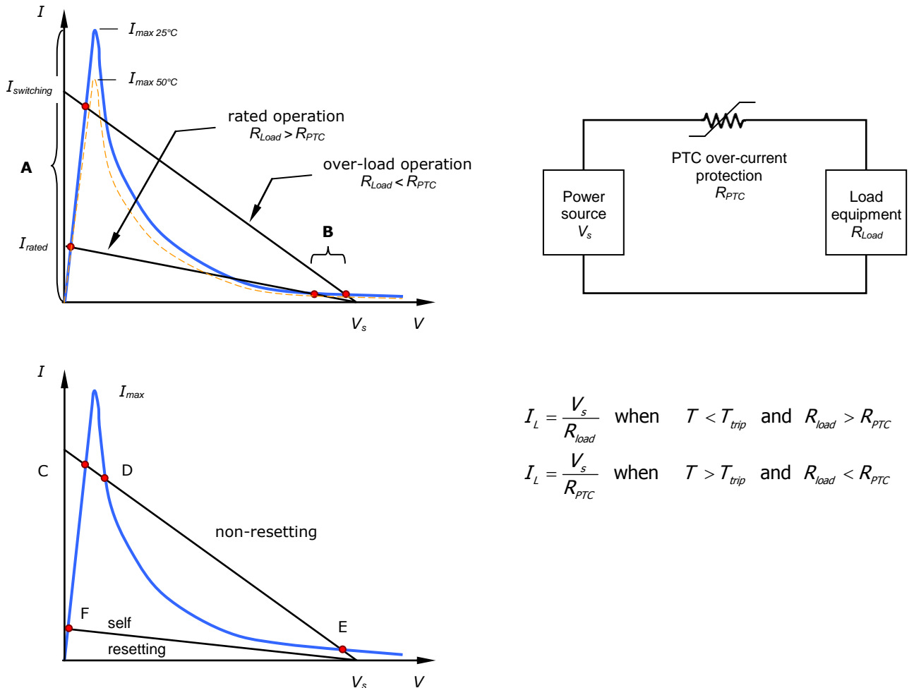
Figure 12.20. Polymeric PTC thermistor circuit operating load line, showing the operating states of a PTC thermistor for over-current protection.
