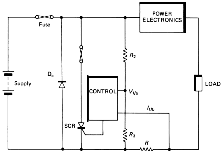
Figure 12.36. An SCR crowbar for overvoltage and over-current protection.
