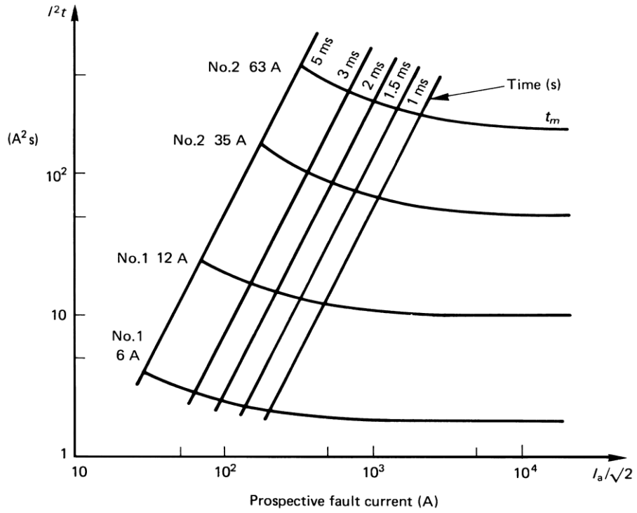
Figure 12.6. Pre-arcing I^2t characteristics of four fuse links.
