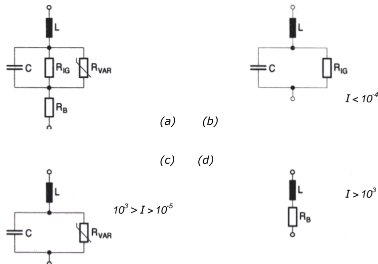
Figure 12.24. Varistor equivalent circuit models: (a) complete model; (b) low current; (c) normal operating region model; and (d) high current model.
