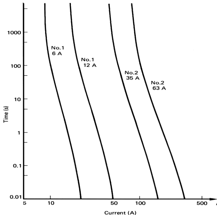
Figure 12.5. Fuse-link time-current characteristics for 4 fuses and symmetrical sinusoidal 50Hz currents.
