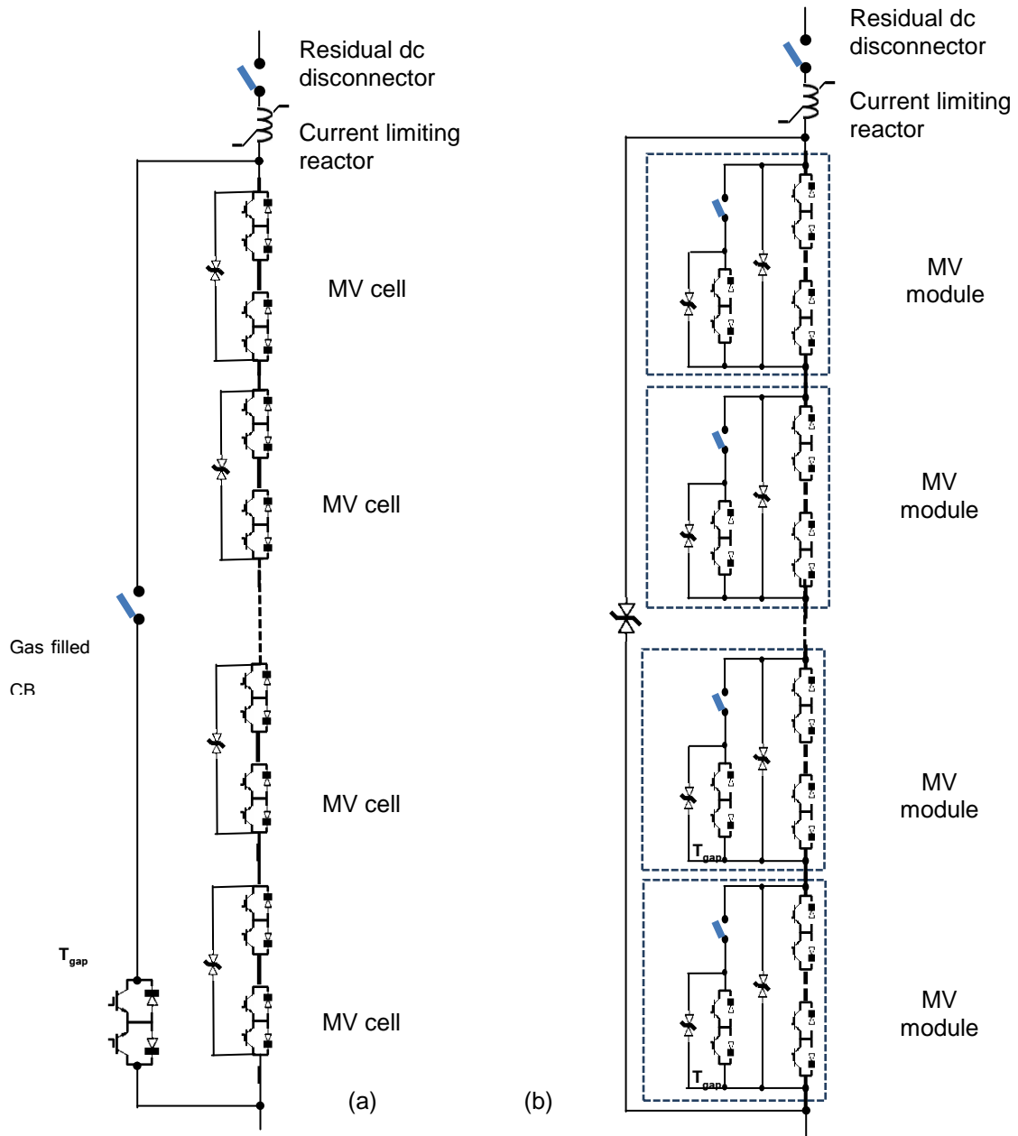
Figure 12.39. Hybrid DCCBs.
