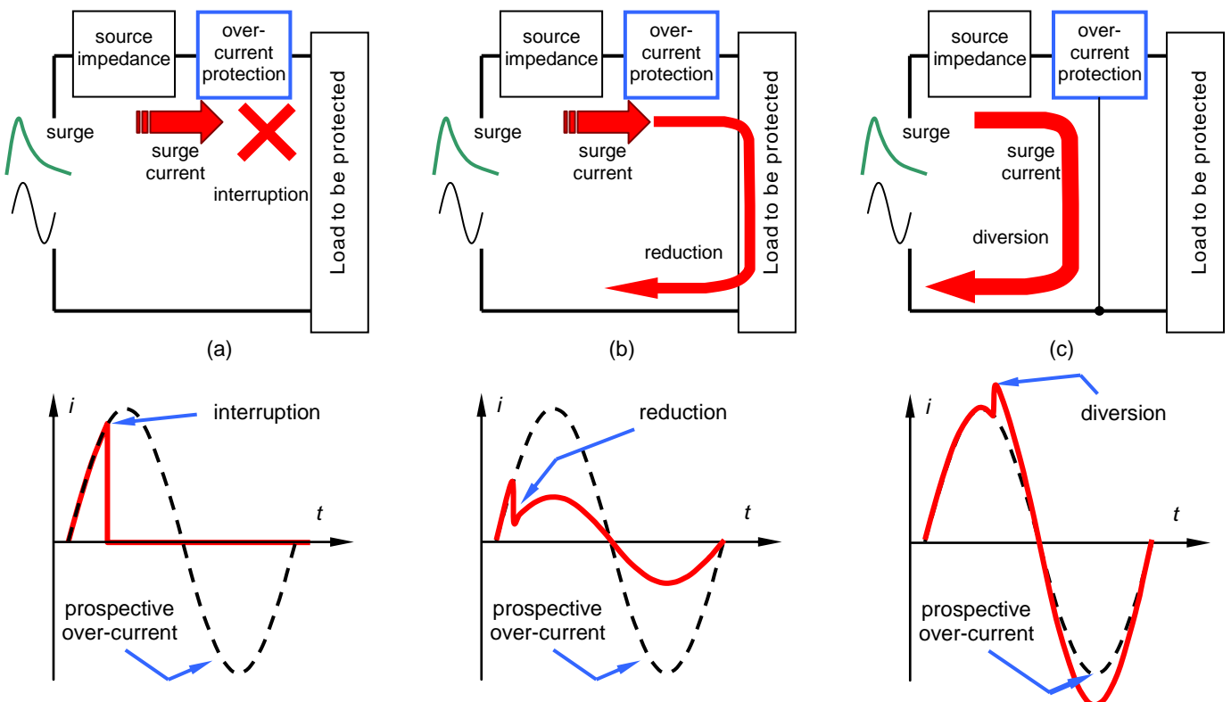
Figure 12.2. Three current limiting mechanisms: (a) current flow interruption, (b) current reduction, and (c) current diversion.
