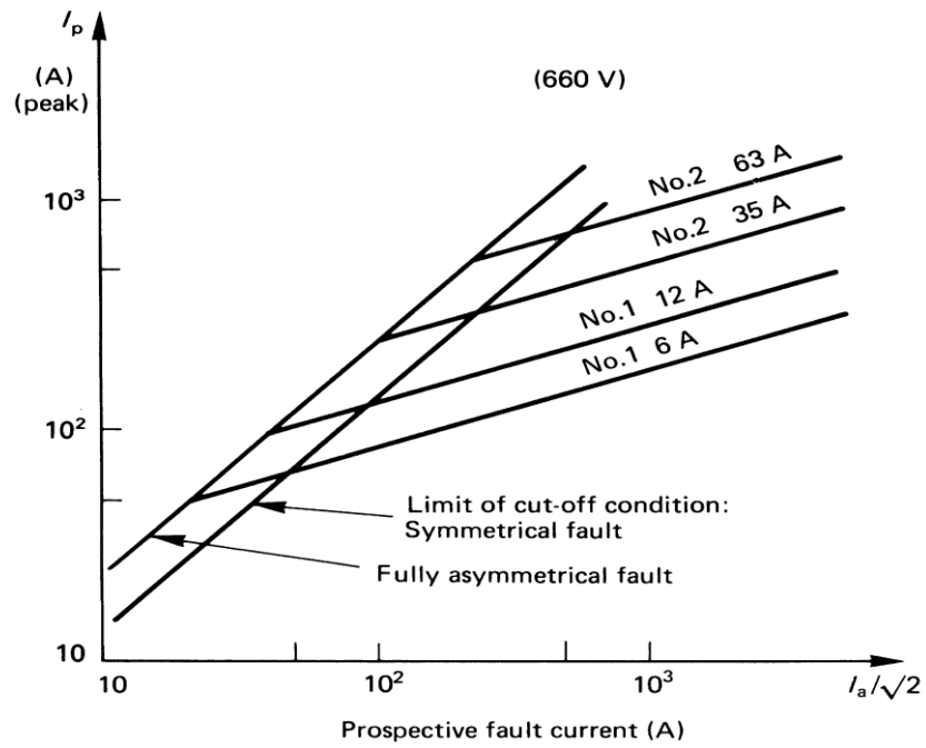
Figure 12.7. Fuse-link cut-off characteristics at 660 V rms.
