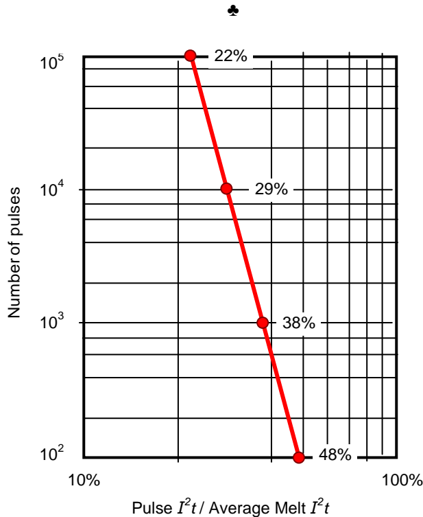
Figure 12.12. Fuse pulse number derating curves, assuming adequate cooling time between pulses.
