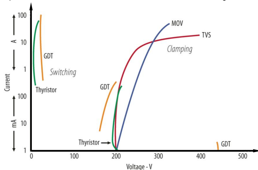
Figure 12.37. The different I - V characteristics of over-voltage protectors.
