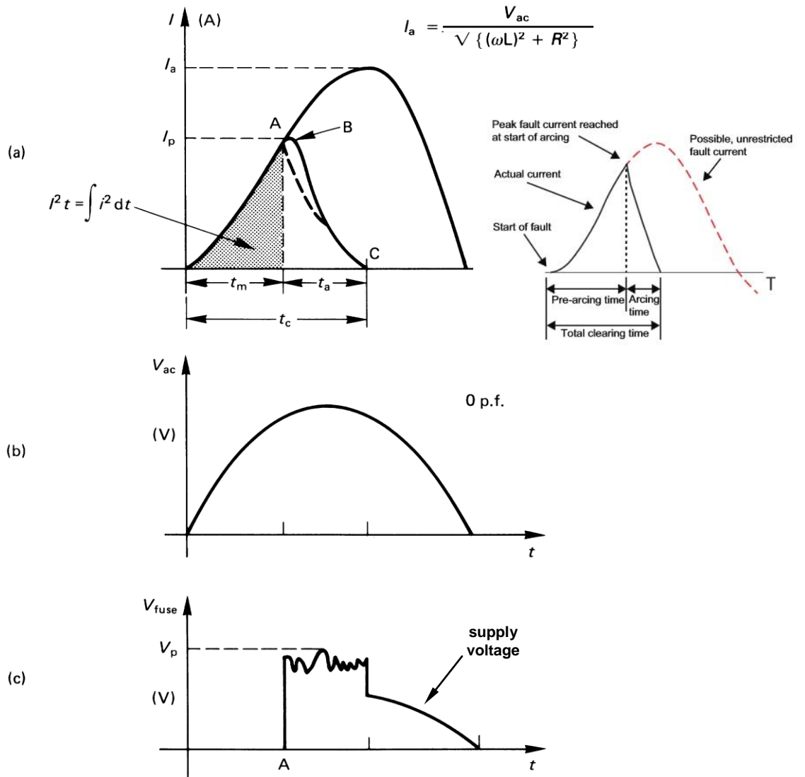
Figure 12.4. Parameters of a fuse link operating: (a) current waveforms; (b) supply voltage; and (c) fuse arcing voltage.
