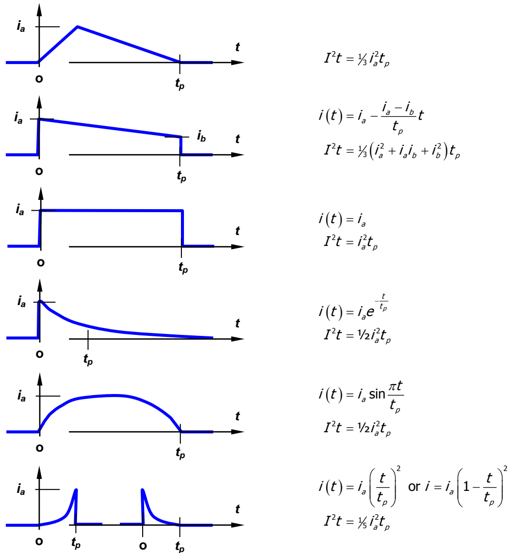
Figure 12.11. Fuse I^2t formula for various current waveforms.
