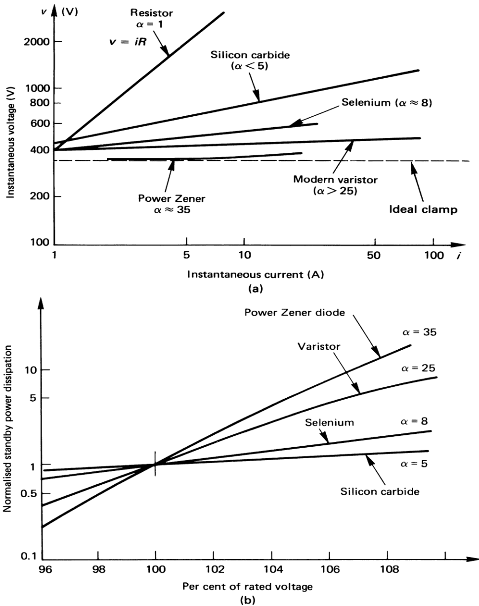
Figure 12.26. (a) The I - V characteristics of four transient voltage suppressor devices, with resistance characteristics for reference and (b) standby power dissipation characteristics showing the higher the \alpha the lower the standby power dissipation.
