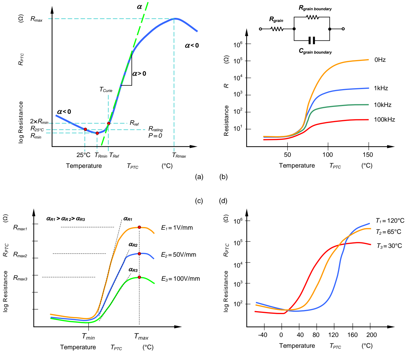
Figure 12.19. PTC ceramic thermistor: (a) R - T characteristics; (b) influence of frequency on R - T characteristics and ac equivalent circuit; (c) influence of electric field strength E (varistor effect) on R - T characteristics; and (d) reference temperature effect on ceramic R - T characteristics.
