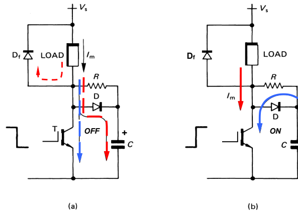
Figure 10.5. Conventional capacitive turn-off snubber showing currents at IGBT transistor: (a) turn-off and (b) turn-on.
