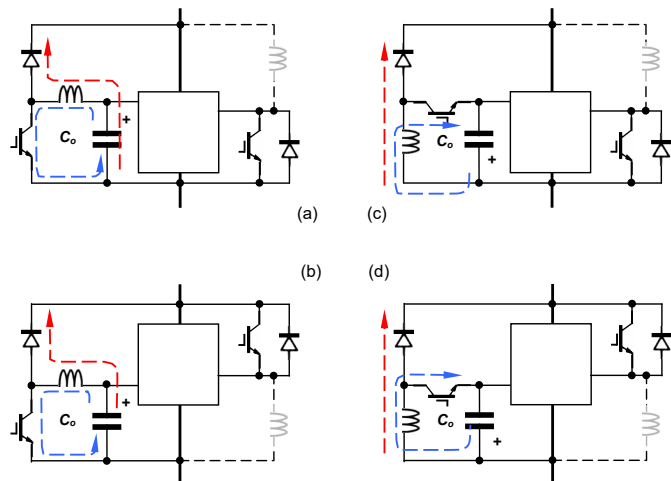
Figure 10.27. Cell active energy recovery from C_o with: (a) and (b) a boost converter and (c) and (d) a buck-boost converter.
