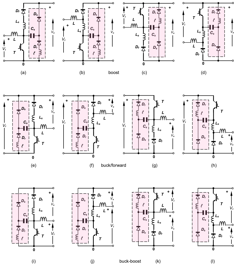
Figure 10.34. Passive energy recovery for inductive turn-on snubber: (a)-(d) a boost converter; (e)-(h) a buck/forward converter; and (i)-(l) a buck-boost converter.
