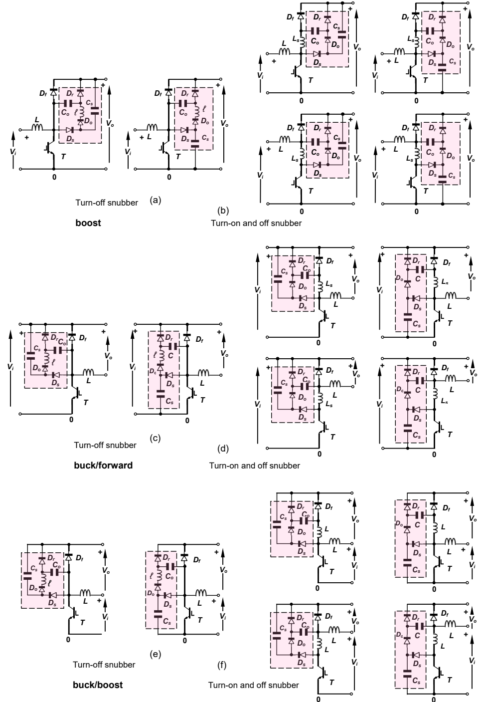
Figure 10.35. Passive energy recovery circuits for the capacitive turn-off snubber and both turn-on and turn-off snubber circuits, for the different types of switched mode converters.
