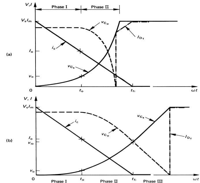
Figure 10.10. Circuit waveforms at switch turn-off with turn-off snubber energy recovery when: (a) the snubber C_s is fully charged before the switch current at turn-off reaches zero and (b) the switch collector current has fallen to zero before the snubber capacitor has charged to V_s .
