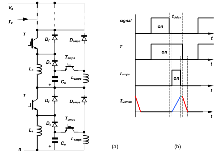
Figure 10.24. Active turn-on snubber energy recovery for series GCT connected, inverter bridge legs: (a) modular cell circuit and (b) timing diagram.
