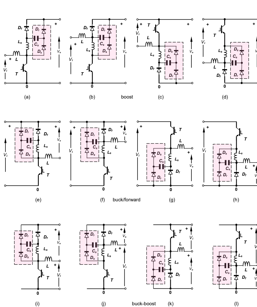
Figure 10.33. Passive energy recovery of freewheel diode recovery energy: (a)-(d) a boost converter; (e)-(h) a buck/forward converter; and (i)-(l) a buck-boost converter.
