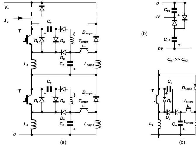
Figure 10.25. Active turn-on and turn-off snubber energy recovery: (a) circuit for series GCT and IGBT inverter bridge legs; (b) high voltage replacement circuit for C_{o1} and (c) reduced component variation of part a.
