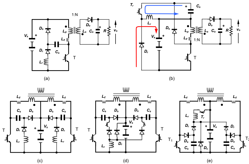
Figure 10.29. Recovery of leakage inductance energy: (a) and (c) passive and (b) (d) and (e) active recovery.
