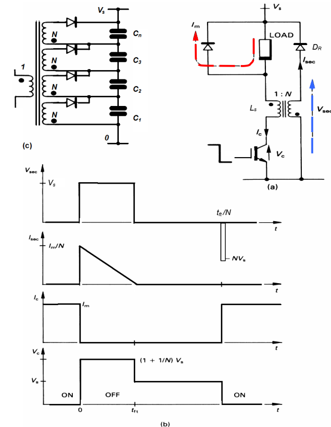
Figure 10.2. Turn-on snubber with snubber energy recovery via a secondary catch winding: (a) circuit diagram; (b) circuit waveforms; and (c) multilevel recovery.
