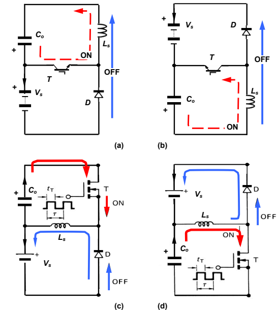
Figure 10.26. Underlying energy recovery circuits when energy in C_o is stored at different potentials: (a) and (b) boost smps recovery and (c) and (d) buck-boost smps recovery.
