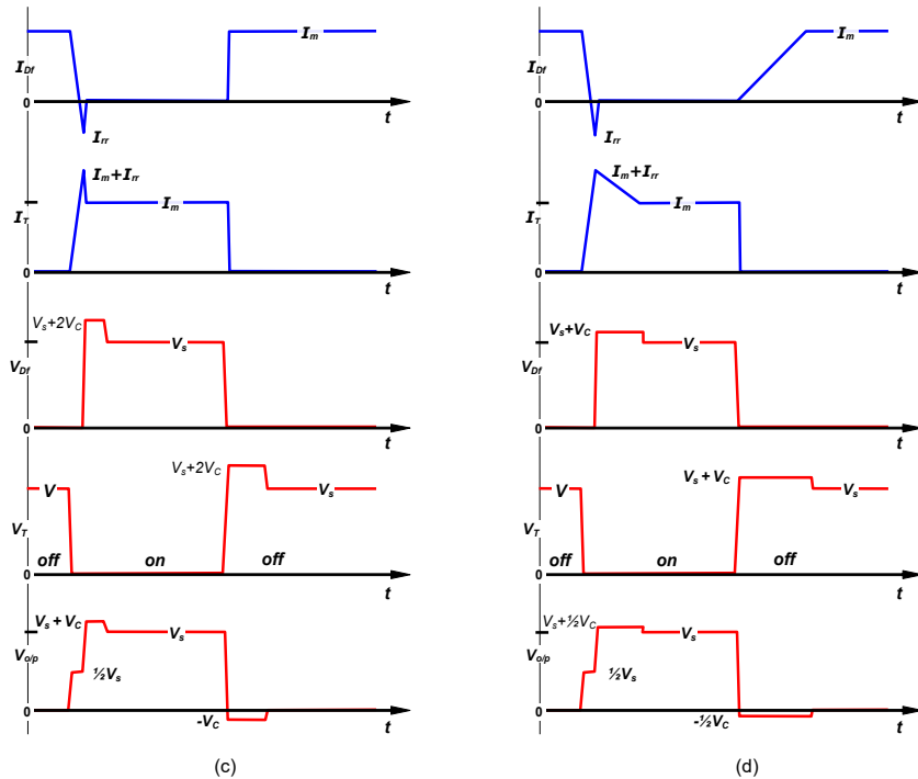
Figure 10.19. Active inductive turn-on snubber energy recovery circuits: (a) multiple single-ended circuit; (b) cross-coupled high frequency circuit; and (c) and (d) respectively circuit waveforms.
