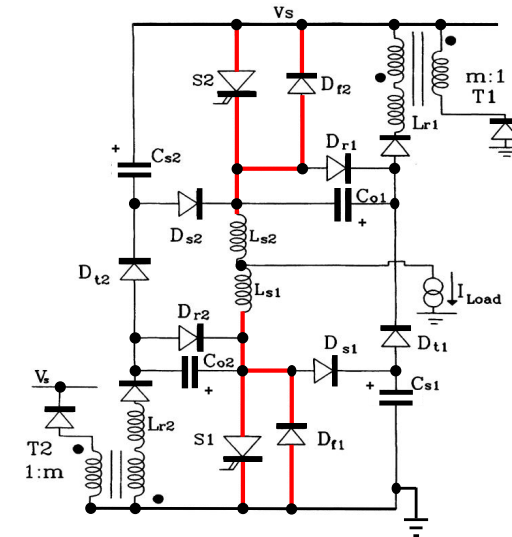
Figure 10.20. Unified, passive snubber energy recovery circuits for GTO and GCT inverter bridge legs.
