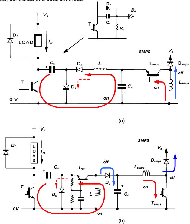
Figure 10.13. Switching circuit for recovering turn-off snubber capacitor energy, and for providing either (a) a negative voltage rail and/or transferring to V_{sv} via a buck-boost smps or (b) a positive voltage rail and/or transferring to V_{sv} via a boost smps.
